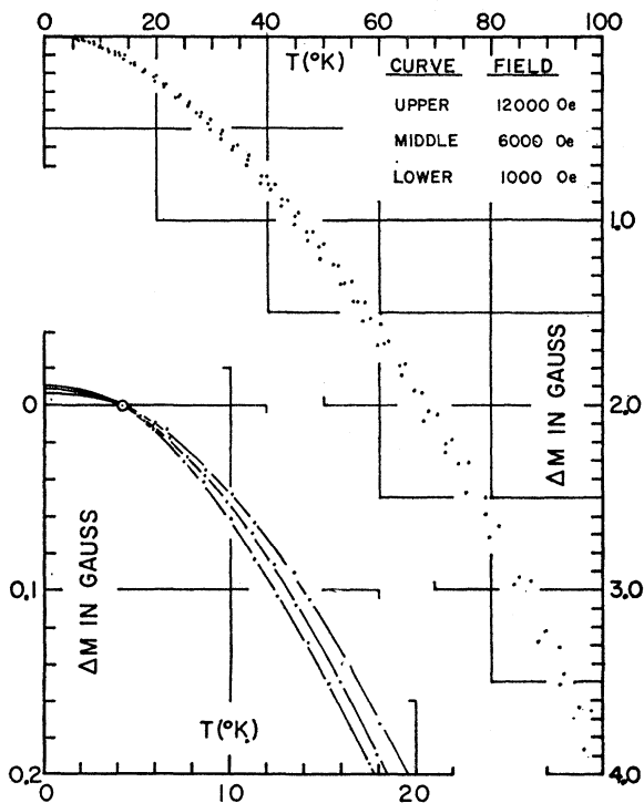
FIG. 1. Observed decreases in magnetization of a single crystal nickel sphere with temperature above 4.2^\circ\text{K} ( \Delta M = 0 at T = 4.2^\circ\text{K} ). The fields indicated were applied parallel to the [111] crystal axis and have been corrected for demagnetizing effects so as to represent internal applied fields. The curves in the lower left corner are the low-temperature portions of the larger curves and are presented on an expanded scale.
