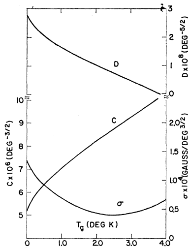
FIG. 4. Results of fitting to spin-wave theory data on the Ni crystal (see Fig. 1) up to 120°K with H=6000 Oe applied parallel to [111] . C and D were allowed to vary independently in the least-squares analysis while T_g was given a range of values from 0 to 4°K. Acceptable values of the parameters must fall within the broad minimum in the \sigma vs T_g plot. The theoretical gap temperature obtained from Eq. (9) is 1.5°K based on g=2.19 , H=6 kOe, M_0=508 G and K_1=-7.5 \times 10^6 ergs/cc.
