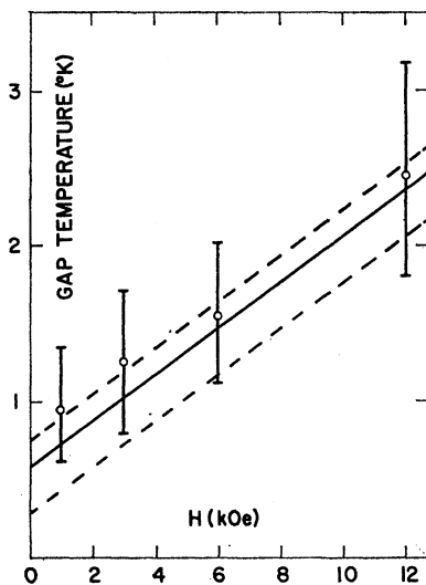
Fig. 6. Comparison of experimental and theoretical values for T_g in Ni as affected by an applied internal field H parallel to [111]. Circles are experimental points obtained from the minima in \sigma vs T_g curves of Fig. 5. Bars indicate accuracy as specified by an arbitrary limit on \sigma of 20% above its minimum. The solid line is given by Eq. (9) for the theoretical effective gap; whereas, the dotted lines are limits of the spread in T_g with \theta_k caused by demagnetization energies of the spin waves. Known values of K_1 and M_0 specify the intercepts while g = 2.19 determines the slope.
